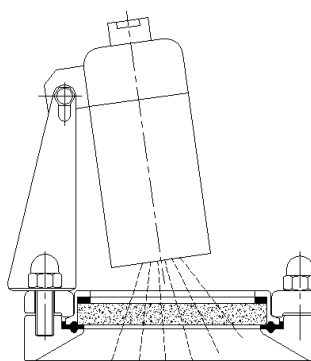
with adjustable hinged bracket
