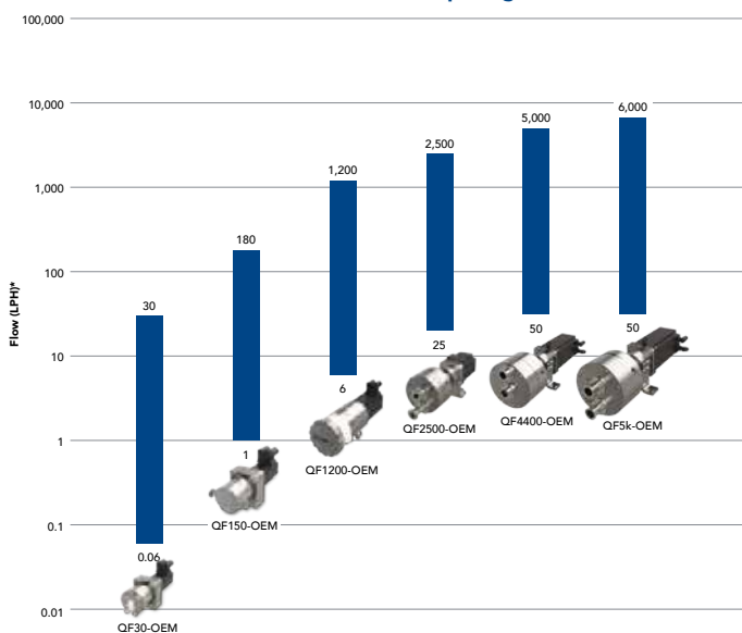
Quattroflow OEM Pump Range
