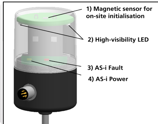
Indicator and operating elements of SISTO-SK-i LED AS-i
